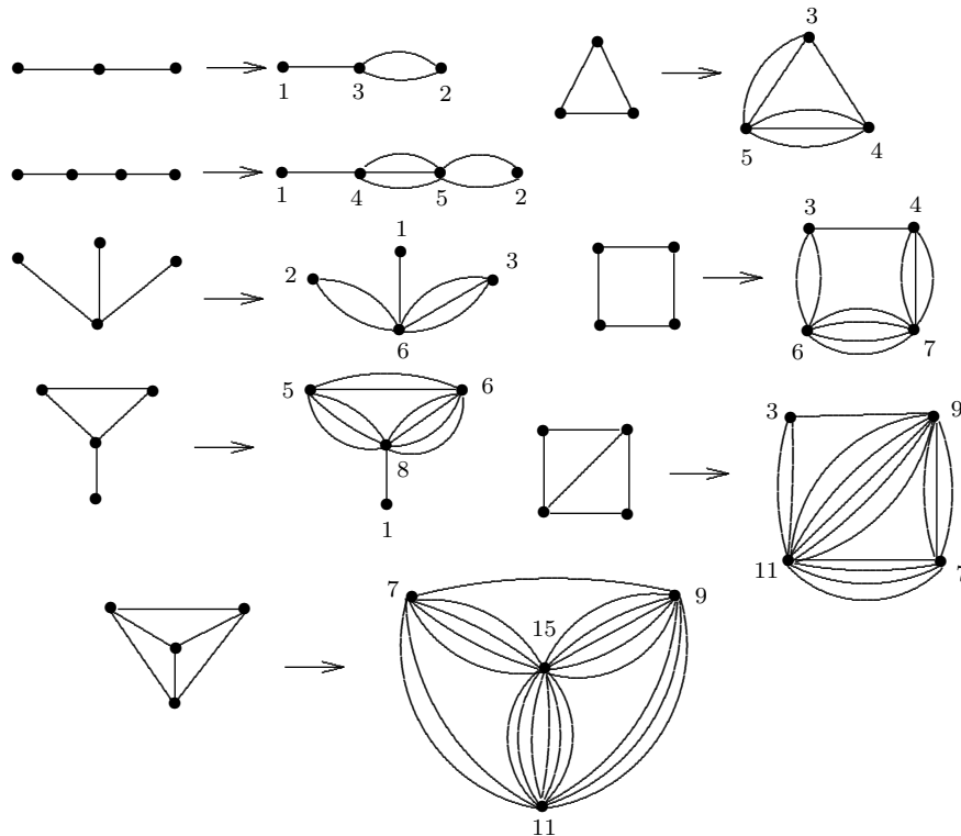
Figure 1.12: Graphs and multigraphs in Exercise 54
