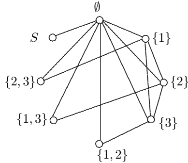
Figure 1.2: The graph G in Exercise 2
