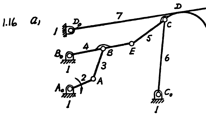
Harvey linkage
